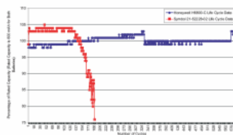
Honeywell H6800-C Versus Symbol 21-52228-02 Life Cycle Testing
